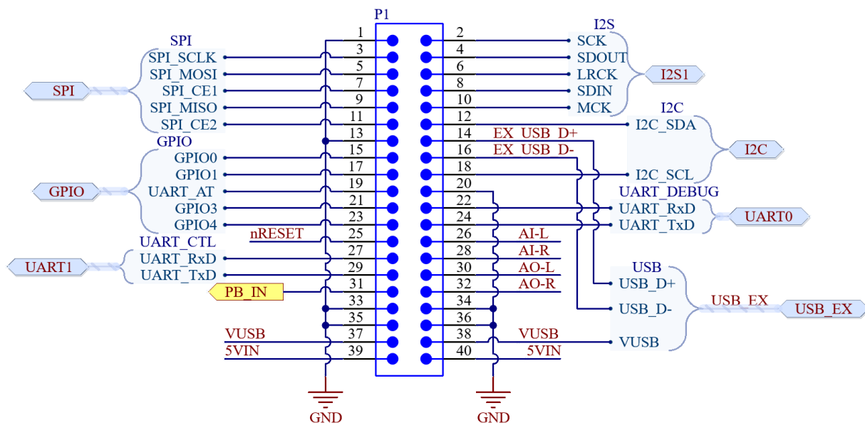
Figure 3 - Aurawave AW100PA-A 40-Pin Connector Pinout
