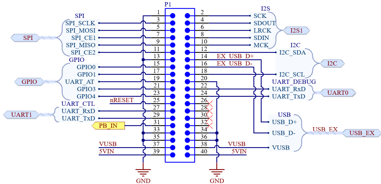
Figure 6 - Aurawave AW100PA-D 40-Pin Connector Pinout
