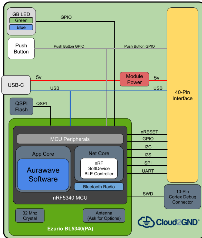
Figure 5 - Aurawave AW100PA-D System Architecture
