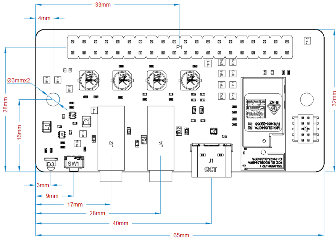
Figure 1 - Aurawave AW100PA-A Dimensions
