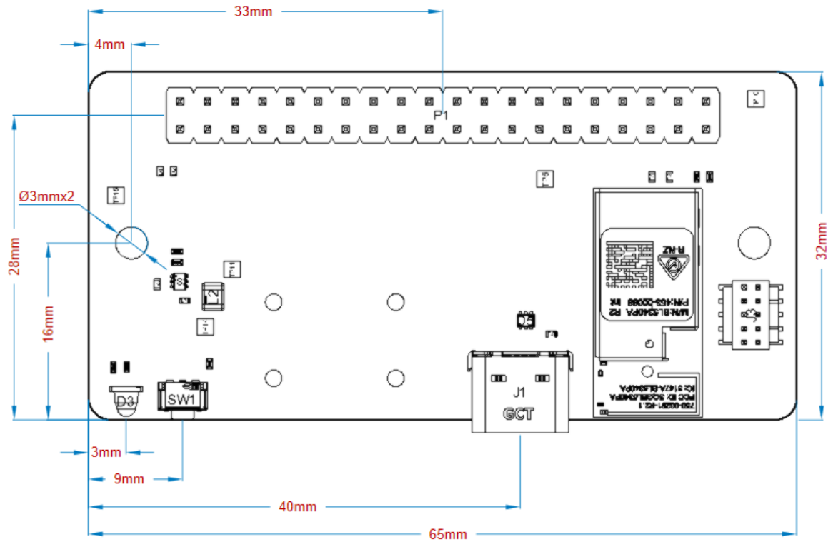
Figure 4 - Aurawave AW100PA-D Dimensions
