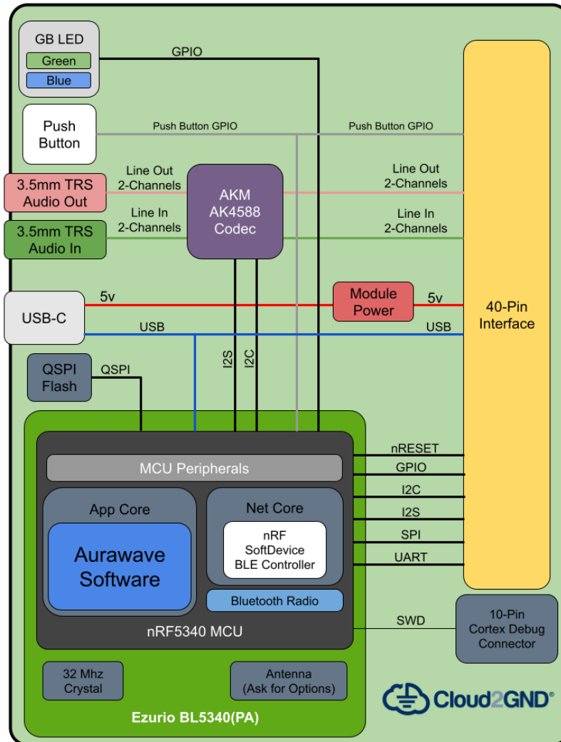
Figure 2 - Aurawave AW100PA-A System Architecture
