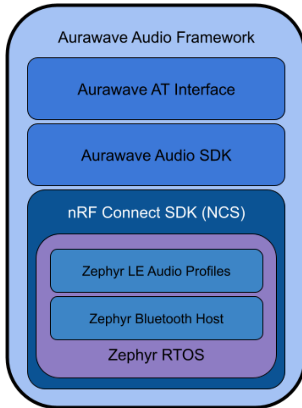
Figure 7 - Aurawave AW100 Software Architecture
